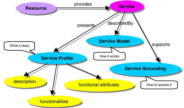
Figure 1: Upper Ontology for Services
