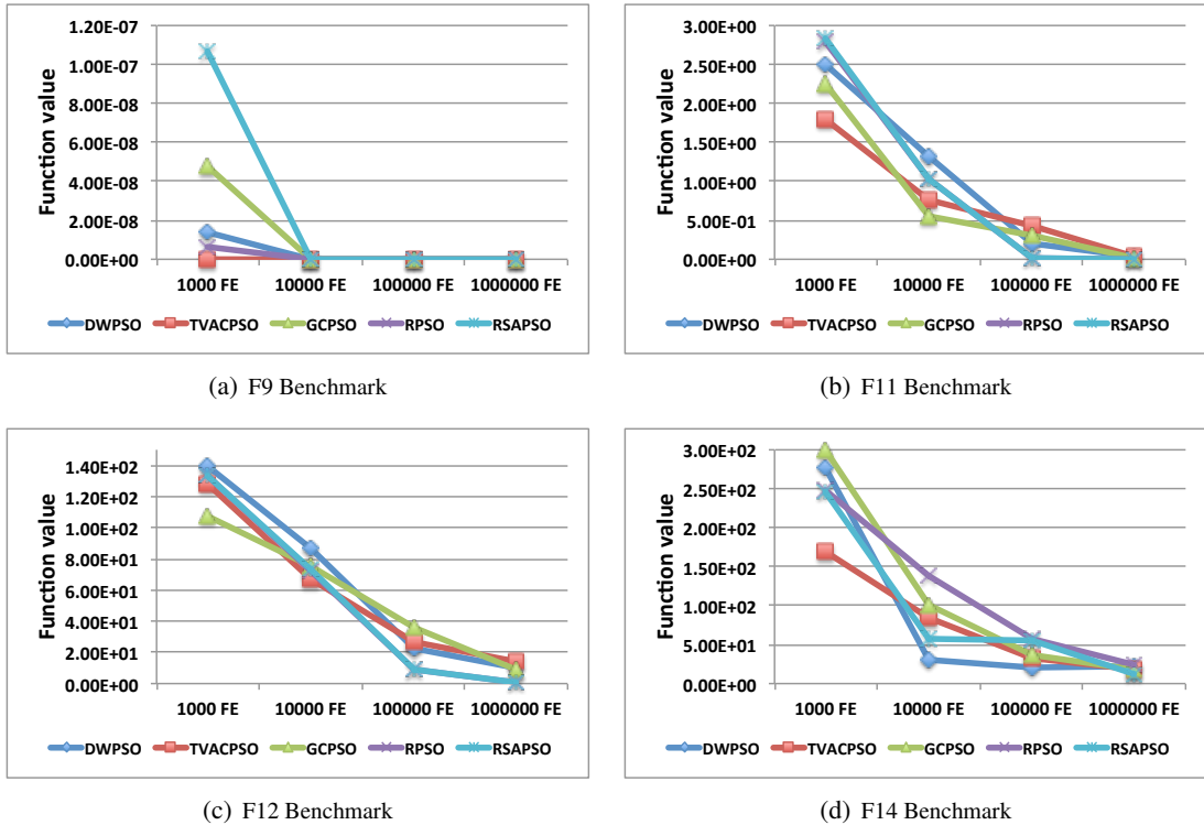
Figure 2: Function value versus FE for different benchmark functions.
